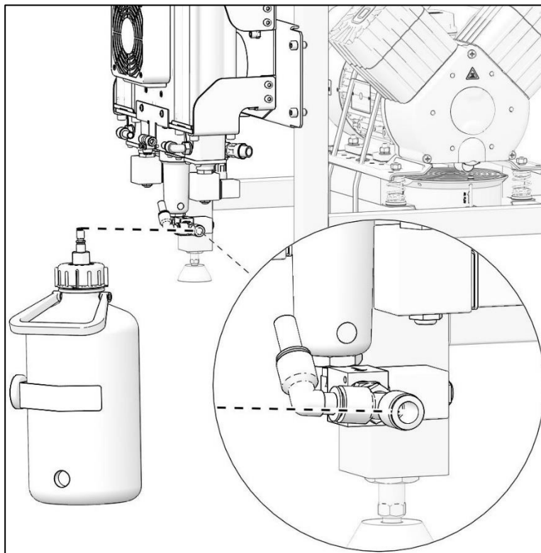
Fig. 16: Check of the condensate collection vessel
