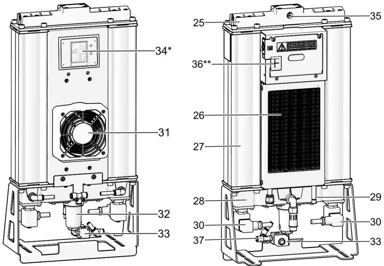
Abb. 2: Adsorptionstrockner
